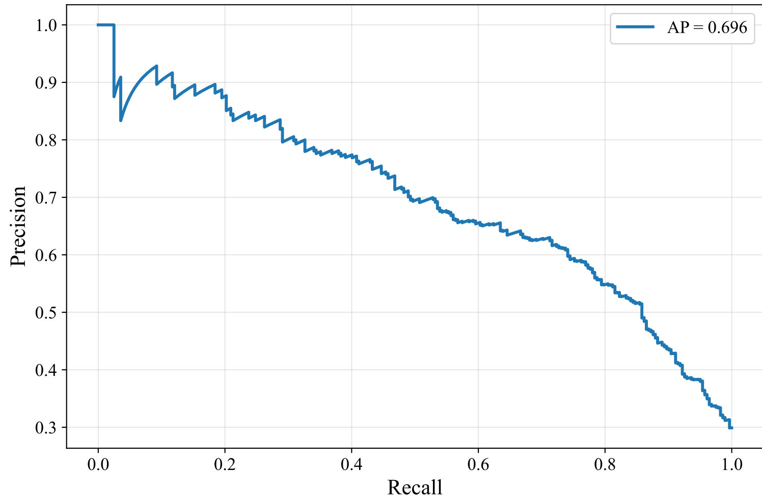
Precision-Recall Curve — ENGLISH_MANUAL (paraphrase-multilingual-mpnet-base-v2, SVM)
