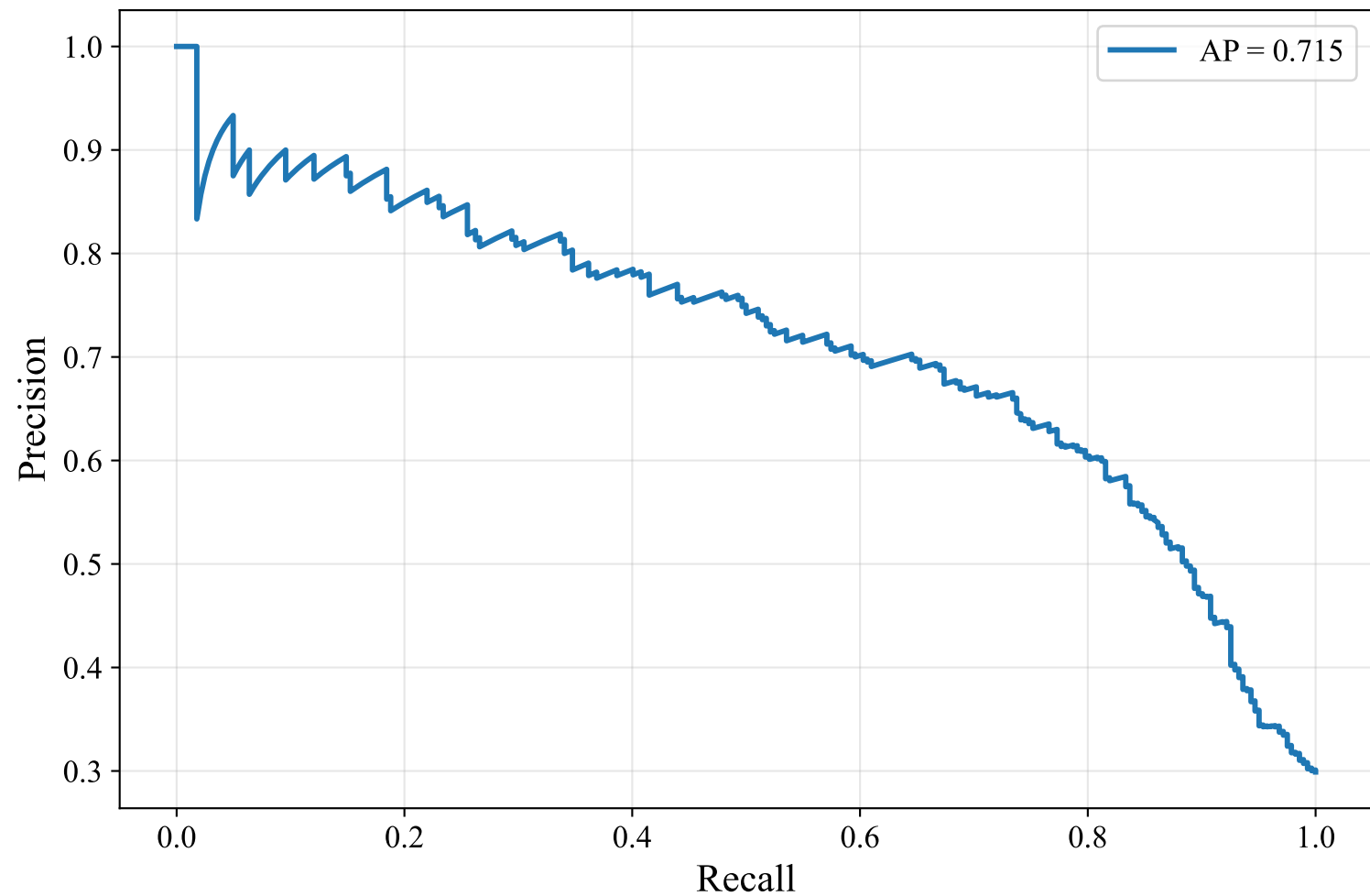
Precision-Recall Curve — ENGLISH_MANUAL (xlm-roberta-base, Random_Forest)
