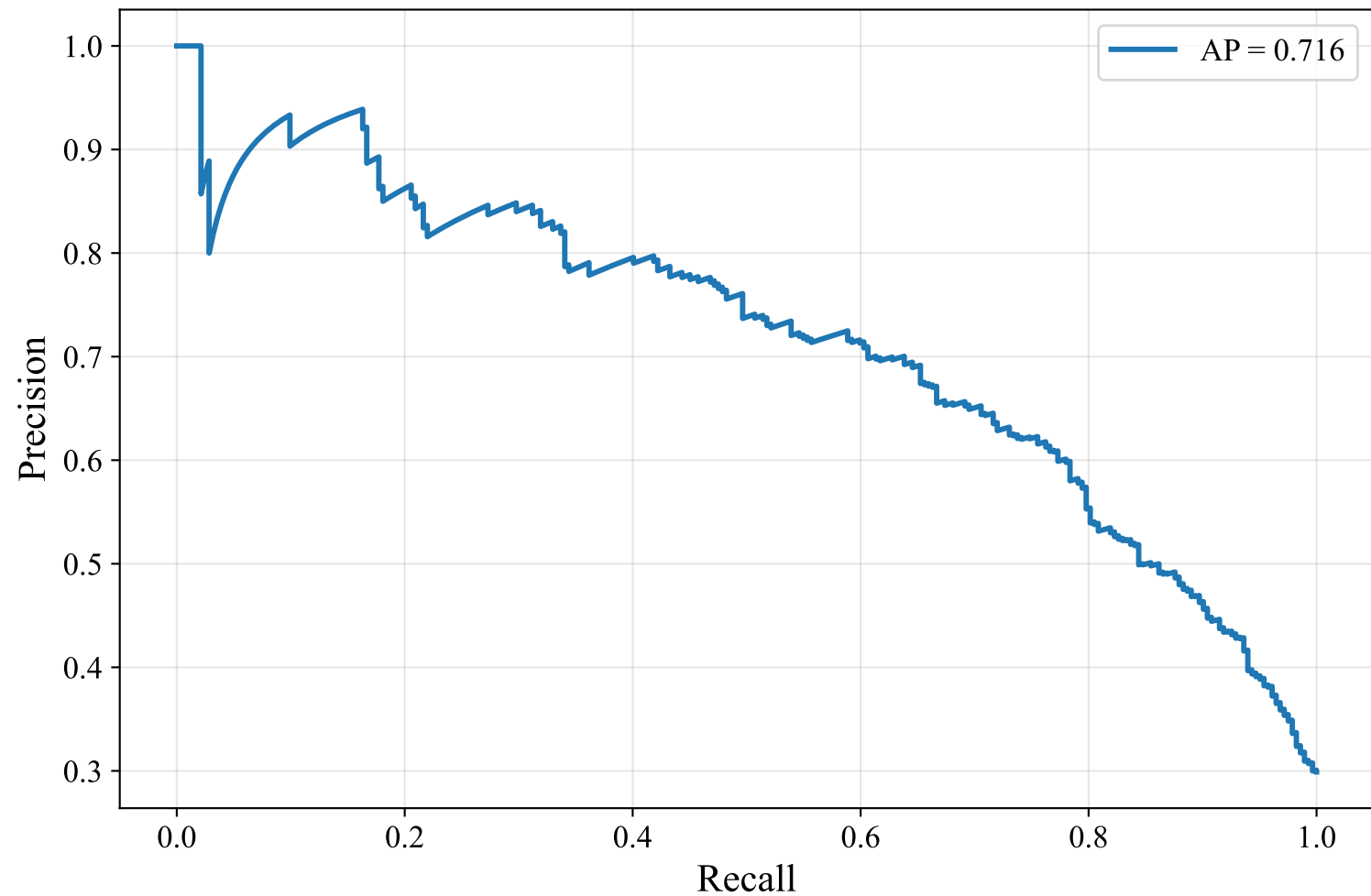
Precision-Recall Curve — ENGLISH_MANUAL (xlm-roberta-base, XGBoost)
