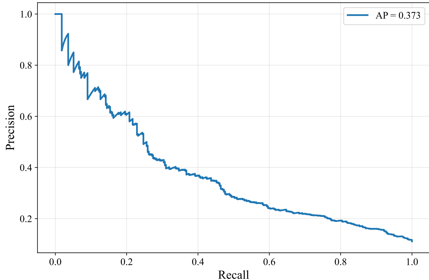
Precision-Recall Curve — GERMAN_MANUAL (paraphrase-multilingual-MiniLM-L12-v2, Random_Forest)
