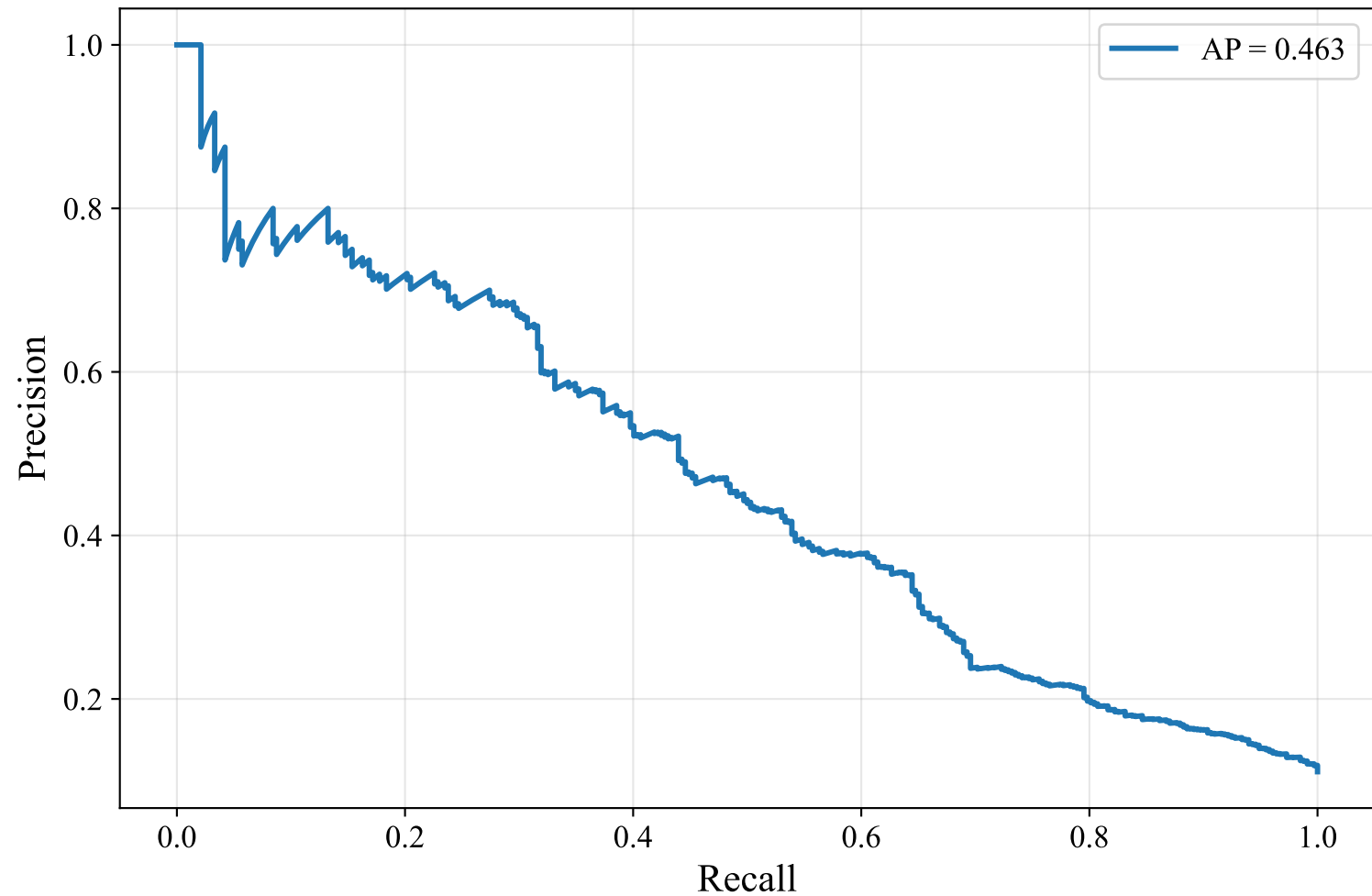
Precision-Recall Curve — GERMAN_MANUAL (xlm-roberta-base, LightGBM)
