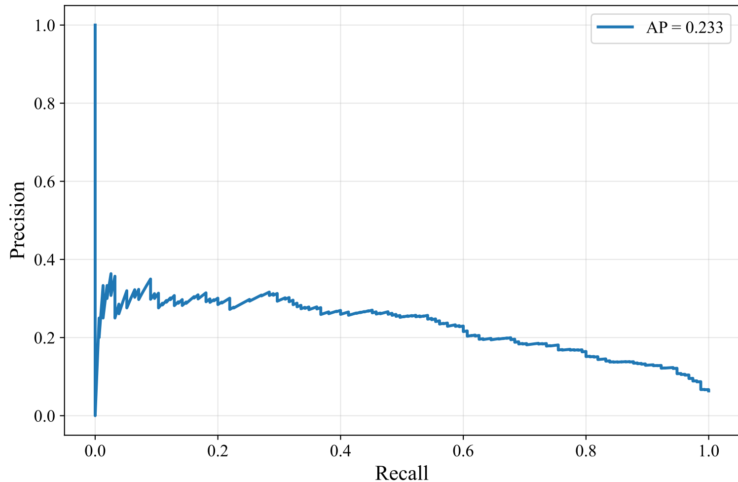
Precision-Recall Curve — SWEDISH_MANUAL (Alibaba-NLP/gte-multilingual-base, Random_Forest)
