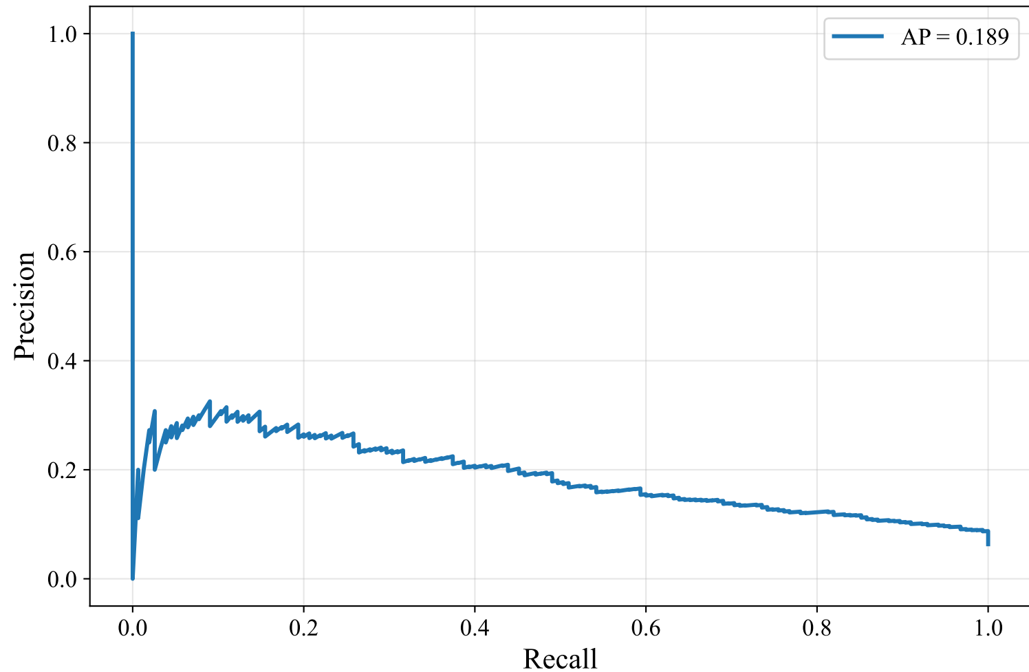
Precision-Recall Curve — SWEDISH_MANUAL (paraphrase-multilingual-MiniLM-L12-v2, XGBoost)
