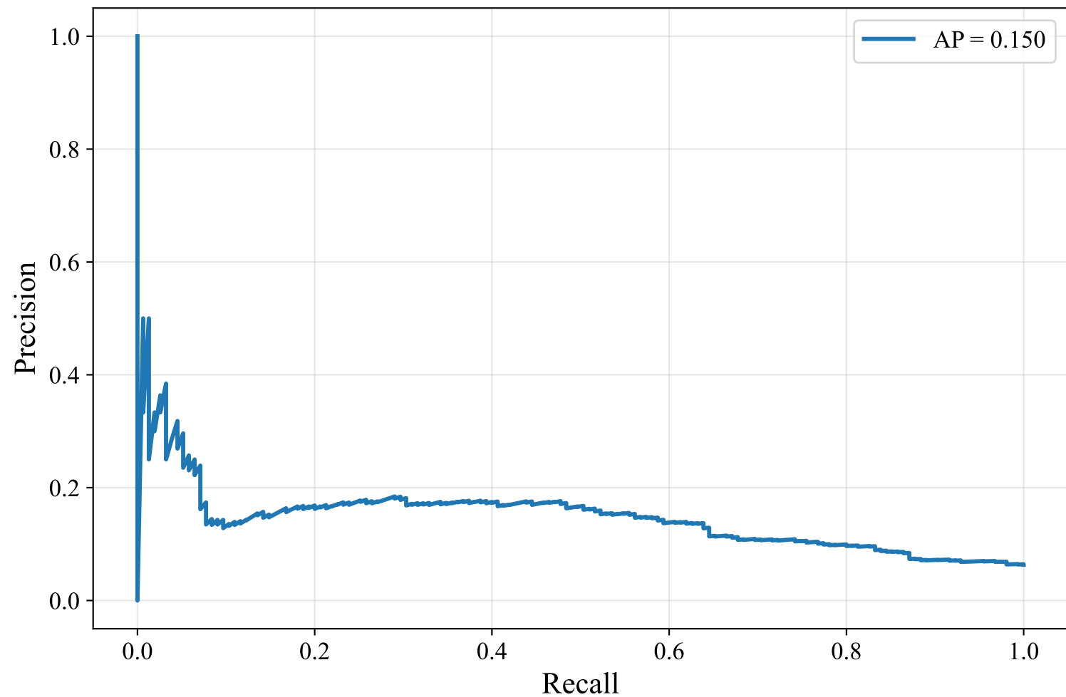
Precision-Recall Curve — SWEDISH_MANUAL (paraphrase-multilingual-mpnet-base-v2, SVM)
