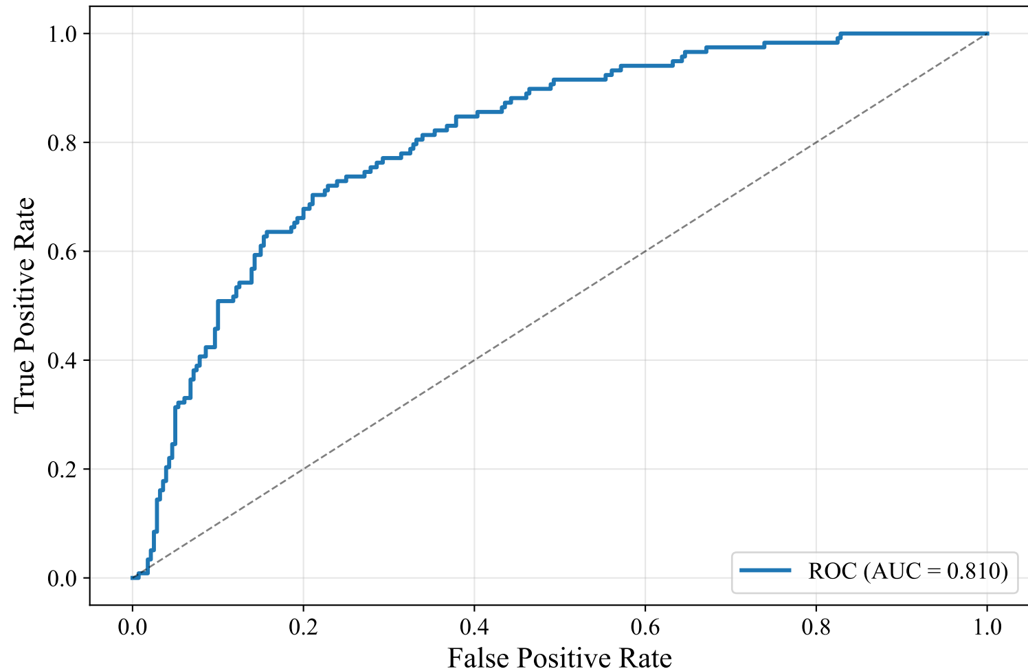
ROC Curve — DUTCH MANUAL (paraphrase-multilingual-mpnet-base-v2, LightGBM)
