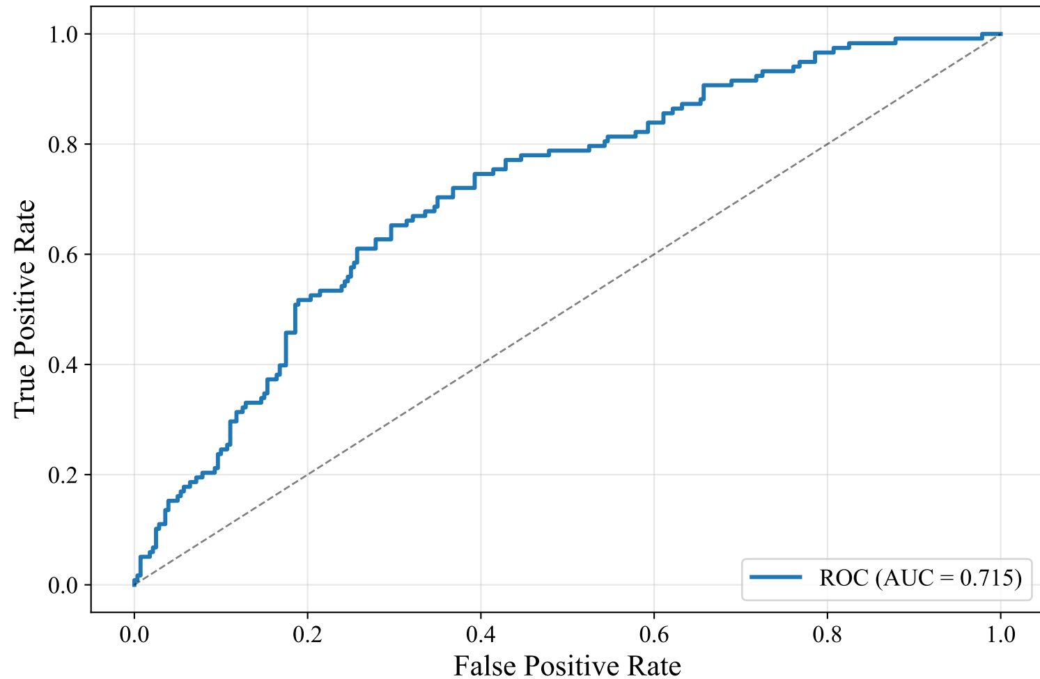
ROC Curve — DUTCH_MANUAL (paraphrase-multilingual-mpnet-base-v2, SVM)
