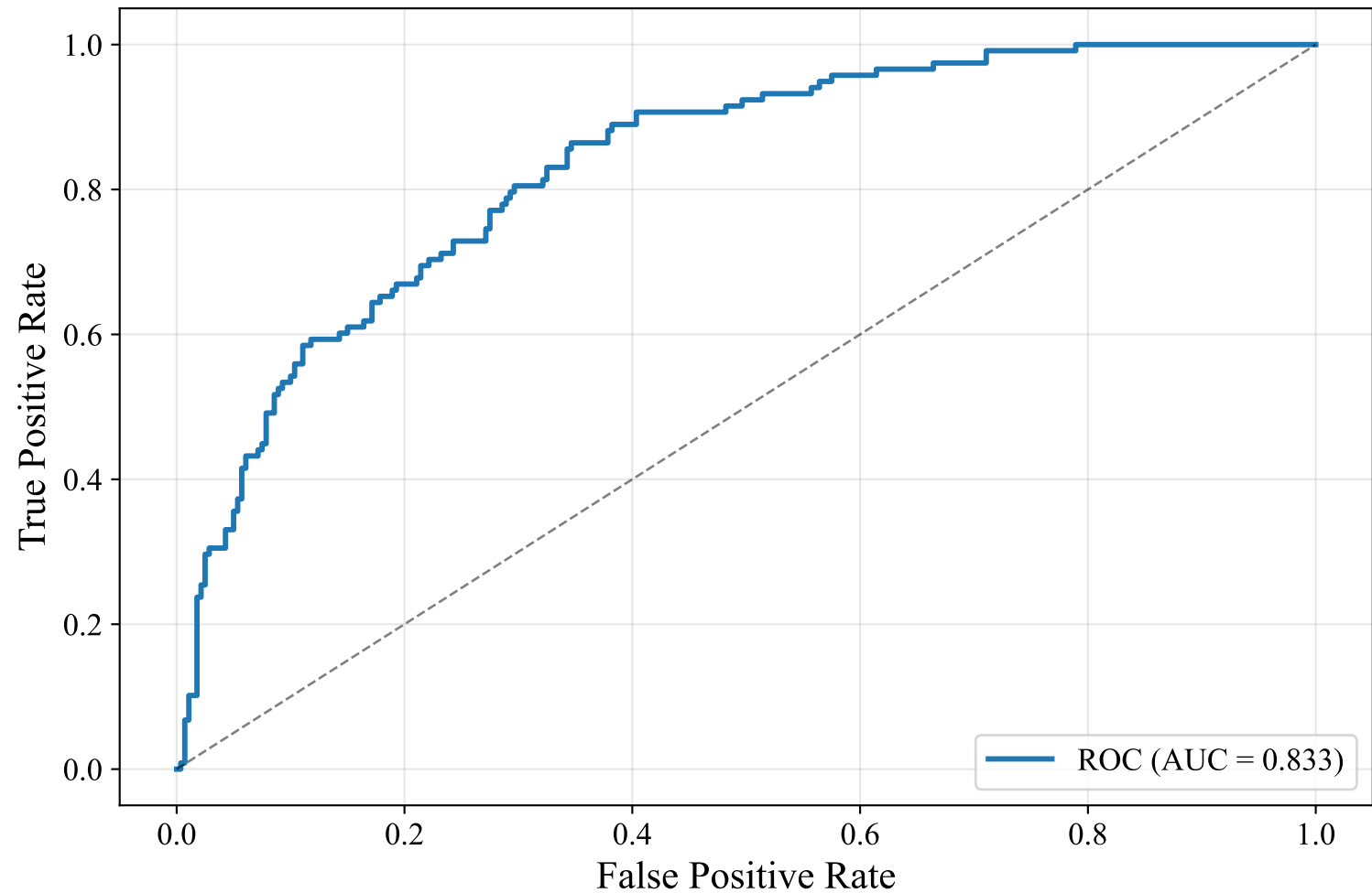
ROC Curve — DUTCH MANUAL (snowflake-arctic-embed-l-v2.0, LightGBM)
