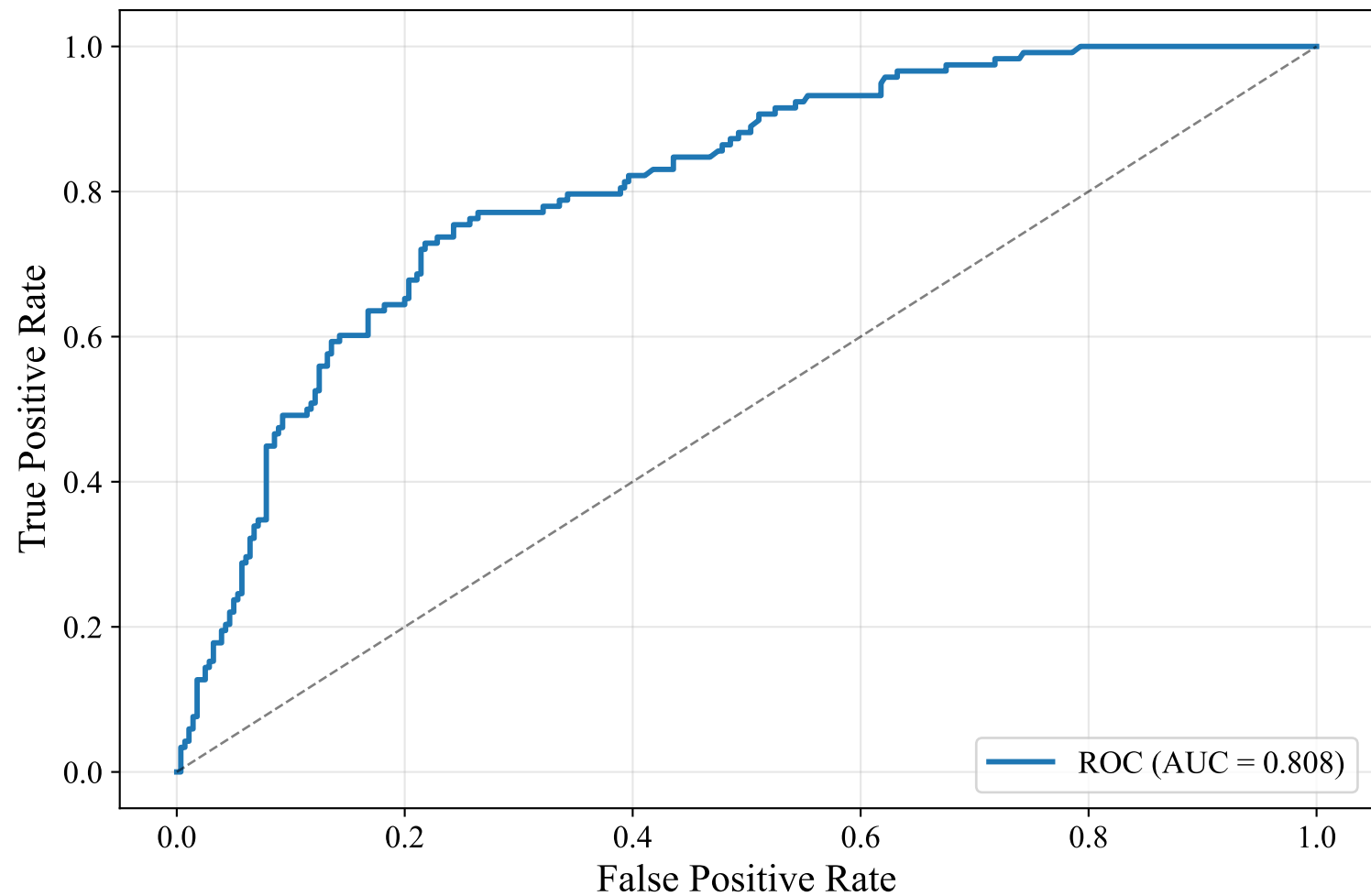
ROC Curve — DUTCH_MANUAL (xlm-roberta-base, Random_Forest)
