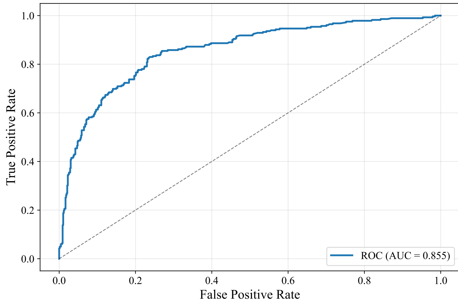
ROC Curve — ENGLISH_MANUAL (Alibaba-NLP/gte-multilingual-base, Random_Forest)
