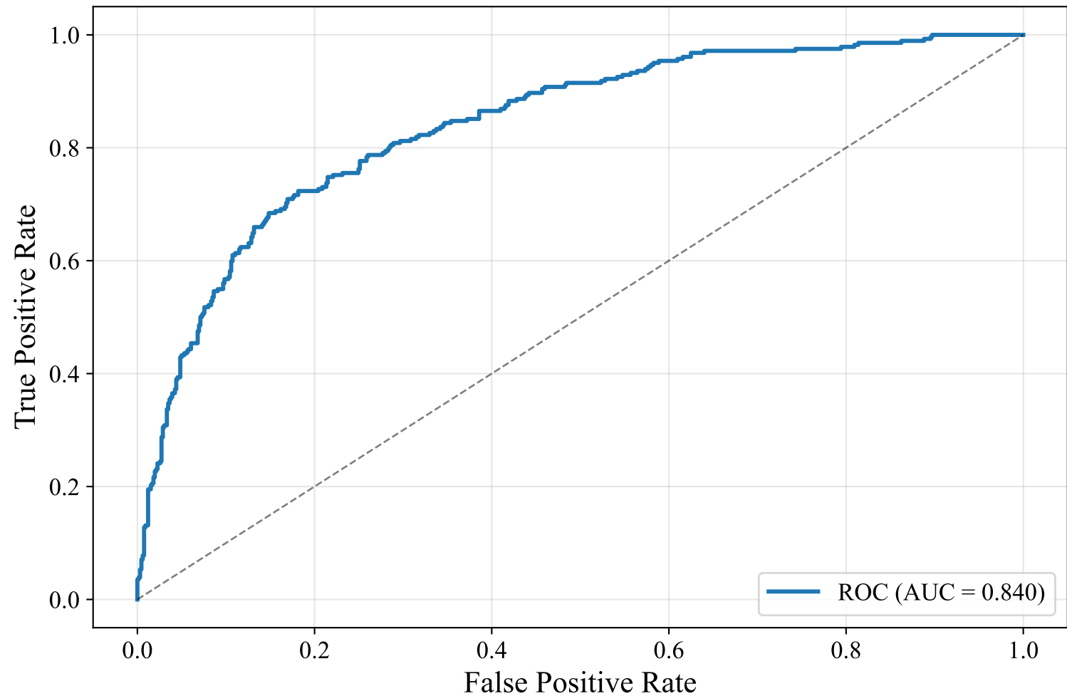
ROC Curve — ENGLISH_MANUAL (bert-base-multilingual-uncased, LightGBM)
