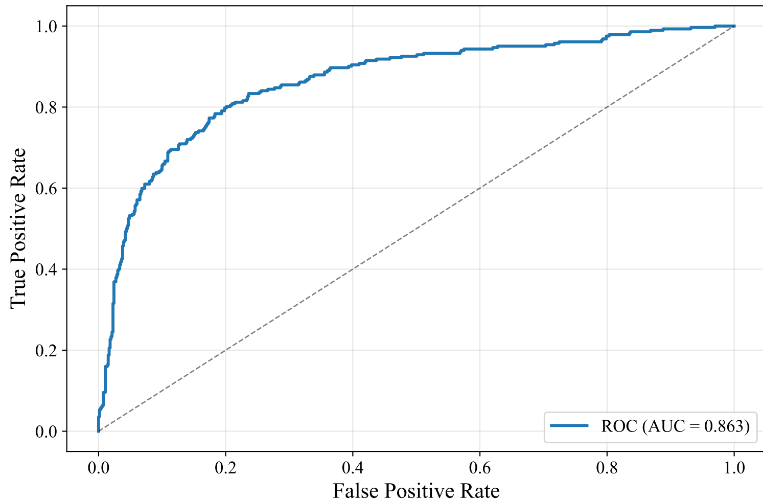
ROC Curve — ENGLISH_MANUAL (intfloat/multilingual-e5-large-instruct, Random_Forest)
