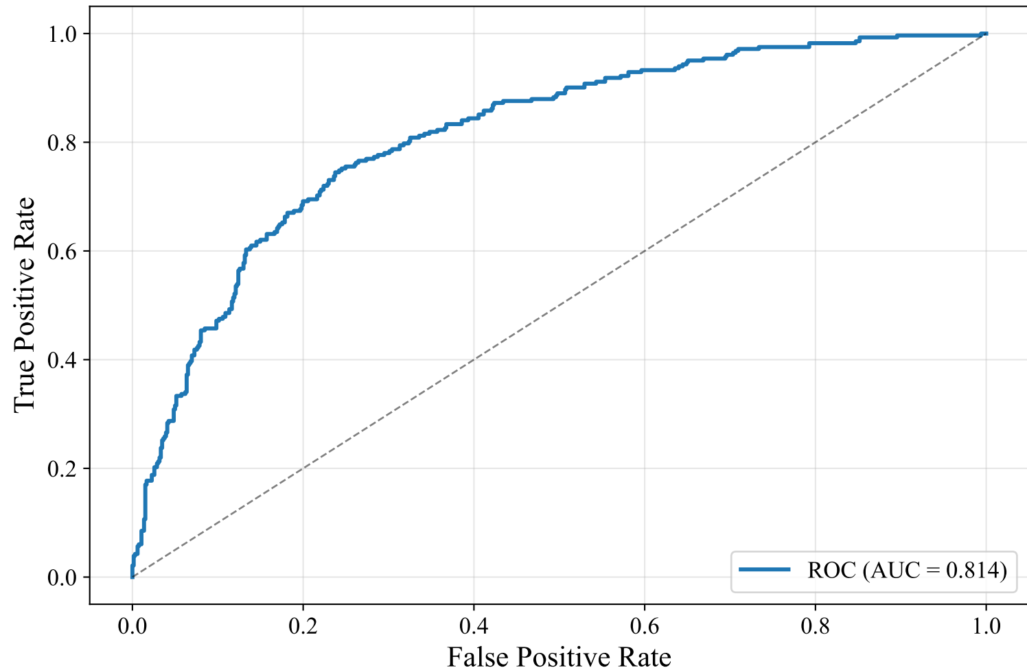
ROC Curve — ENGLISH_MANUAL (intfloat/multilingual-e5-large-instruct, SVM)
