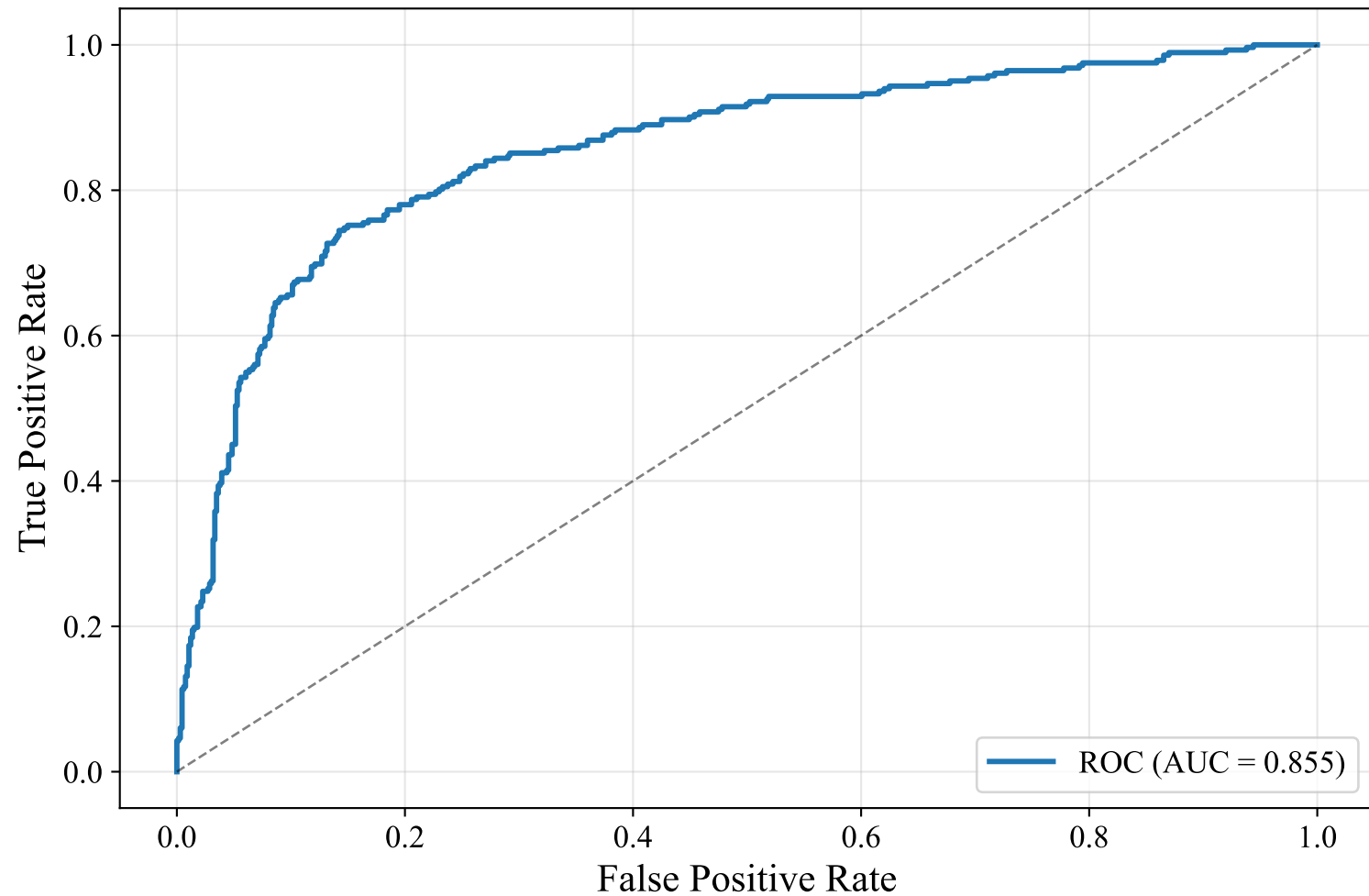
ROC Curve — ENGLISH_MANUAL (snowflake-arctic-embed-l-v2.0, LightGBM)
