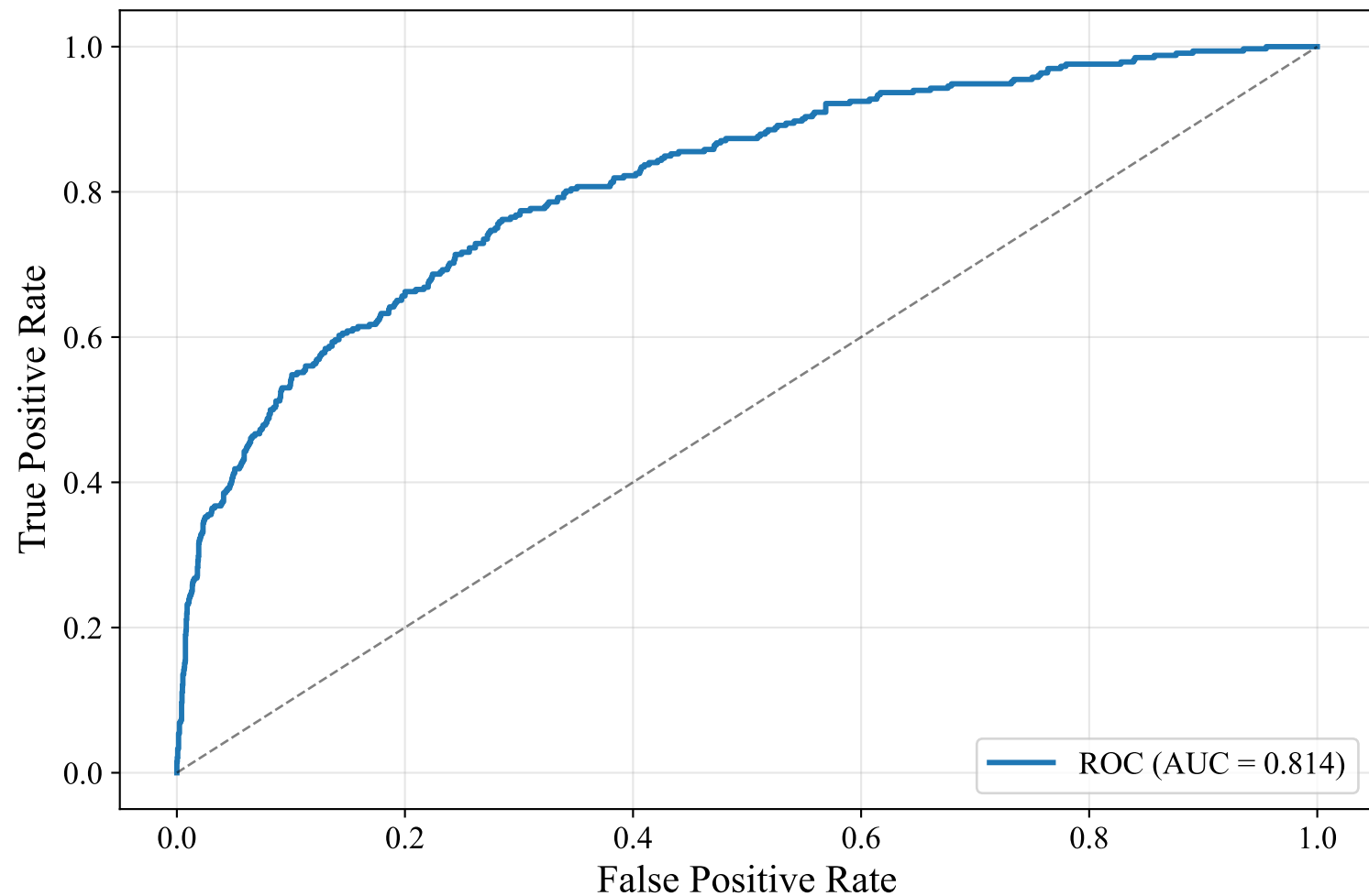
ROC Curve — GERMAN_MANUAL (bert-base-multilingual-uncased, LightGBM)
