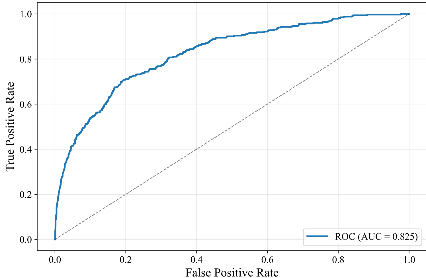
ROC Curve — GERMAN_MANUAL (bert-base-multilingual-uncased, XGBoost)
