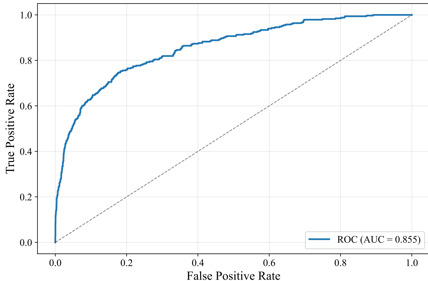
ROC Curve — GERMAN_MANUAL (intfloat/multilingual-e5-large-instruct, LightGBM)
