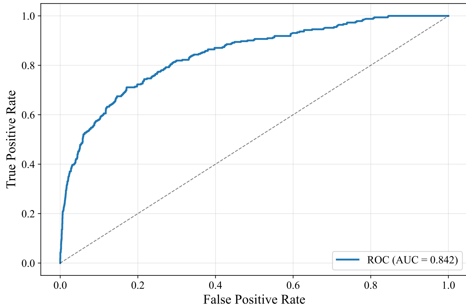
ROC Curve — GERMAN_MANUAL (snowflake-arctic-embed-l-v2.0, Random_Forest)
