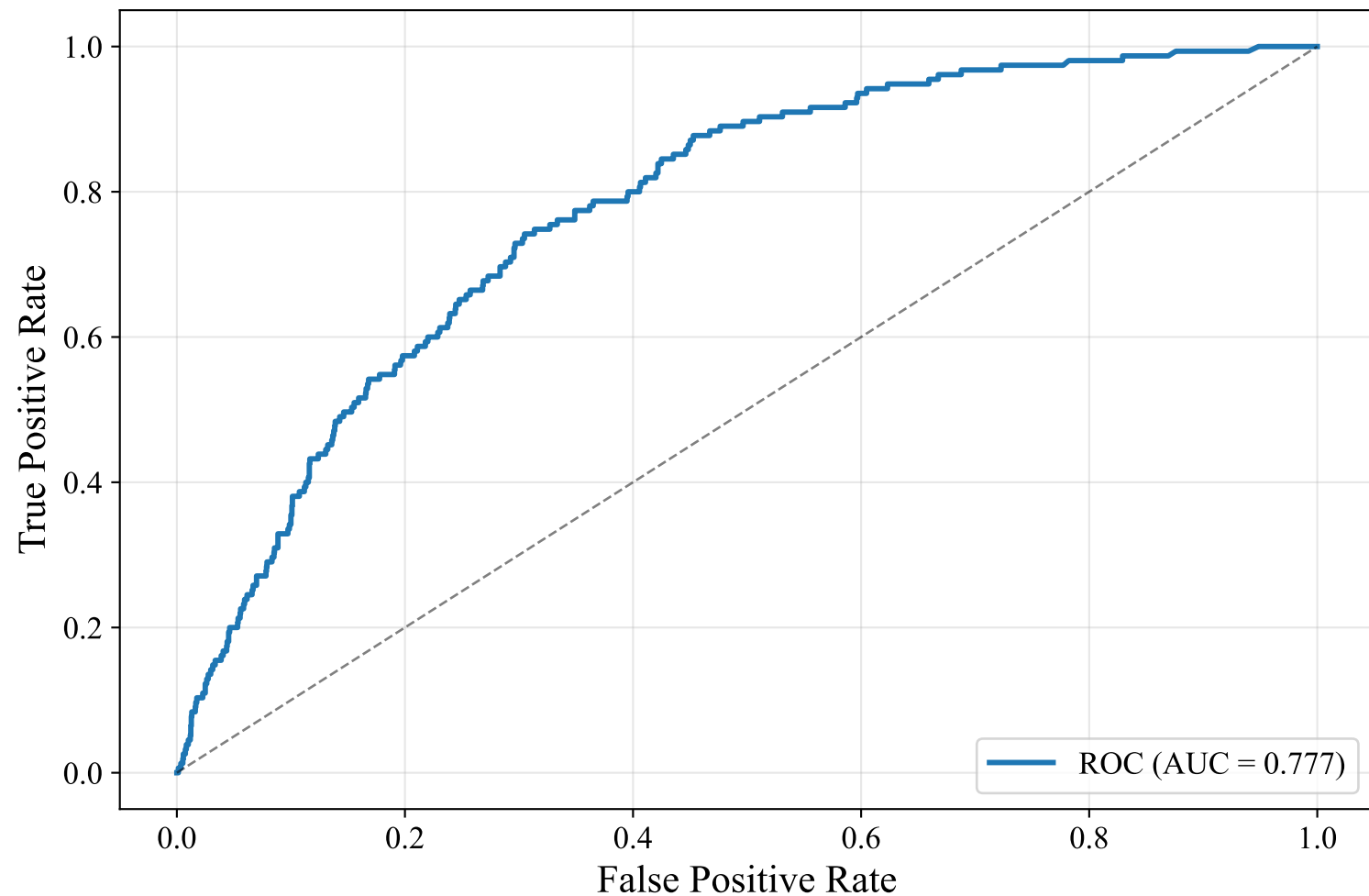
ROC Curve — SWEDISH_MANUAL (bert-base-multilingual-uncased, Random_Forest)
