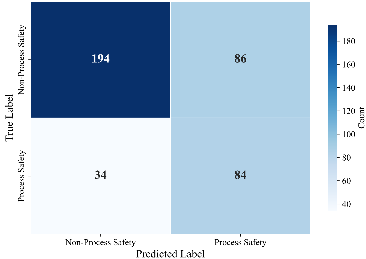
Confusion Matrix — DUTCH_MANUAL (bert-base-multilingual-uncased, Voting_Ensemble)
