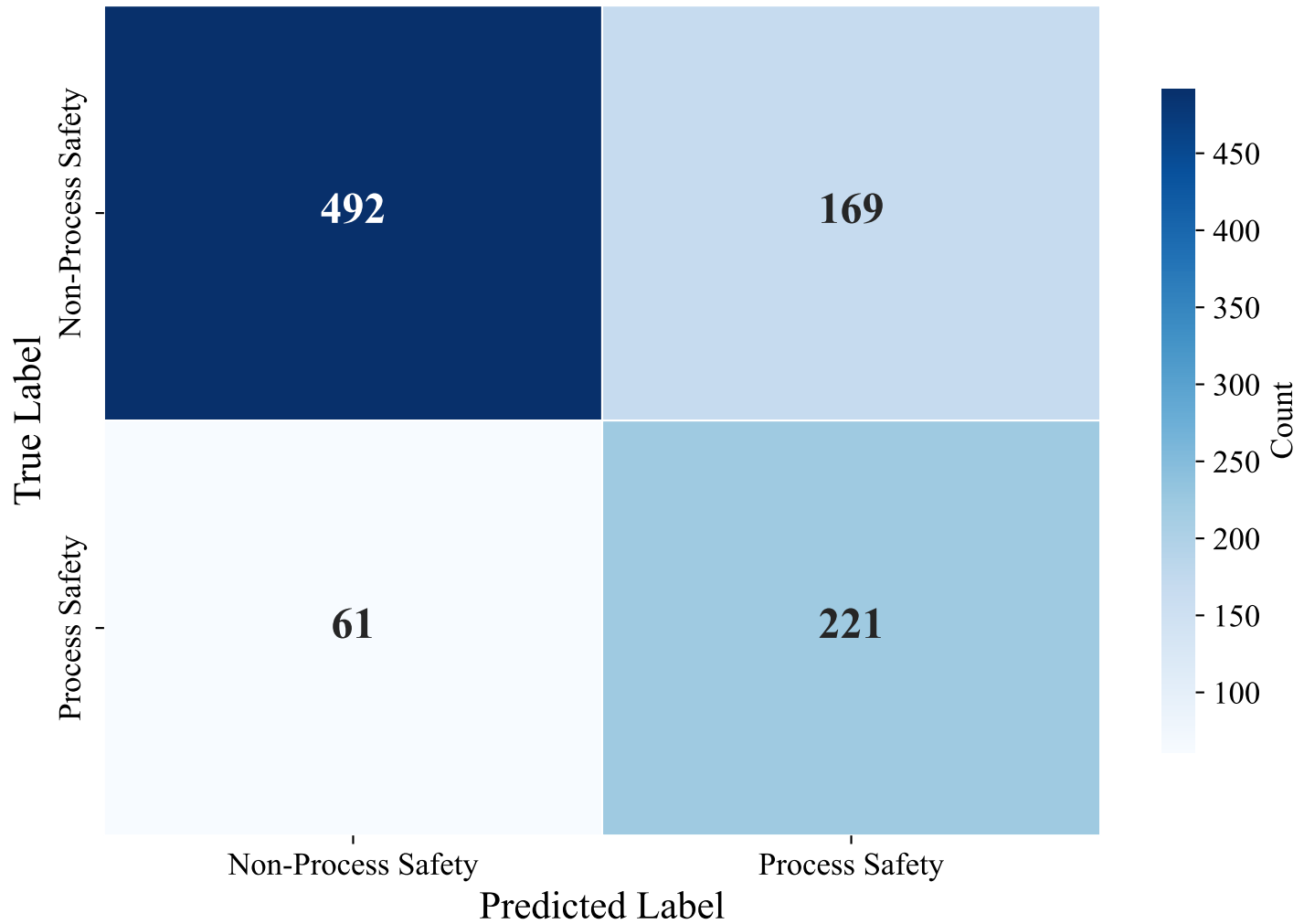
Confusion Matrix — ENGLISH_MANUAL (bert-base-multilingual-uncased, XGBoost)
