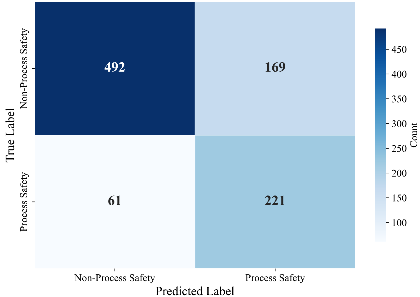
Confusion Matrix — ENGLISH_MANUAL (bert-base-multilingual-uncased, XGBoost_Optimized)
