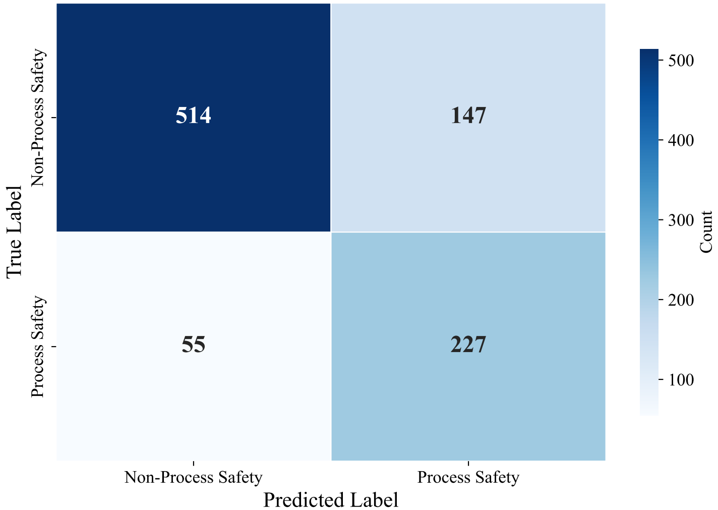
Confusion Matrix — ENGLISH_MANUAL (paraphrase-multilingual-mpnet-base-v2, LightGBM)
