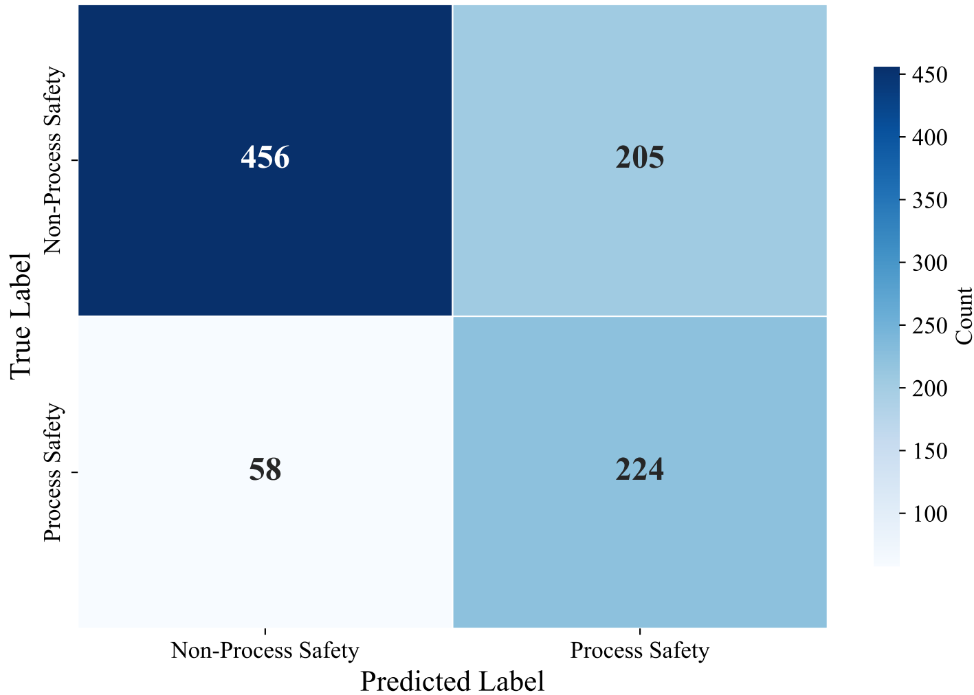
Confusion Matrix — ENGLISH_MANUAL (xlm-roberta-base, Random_Forest)
