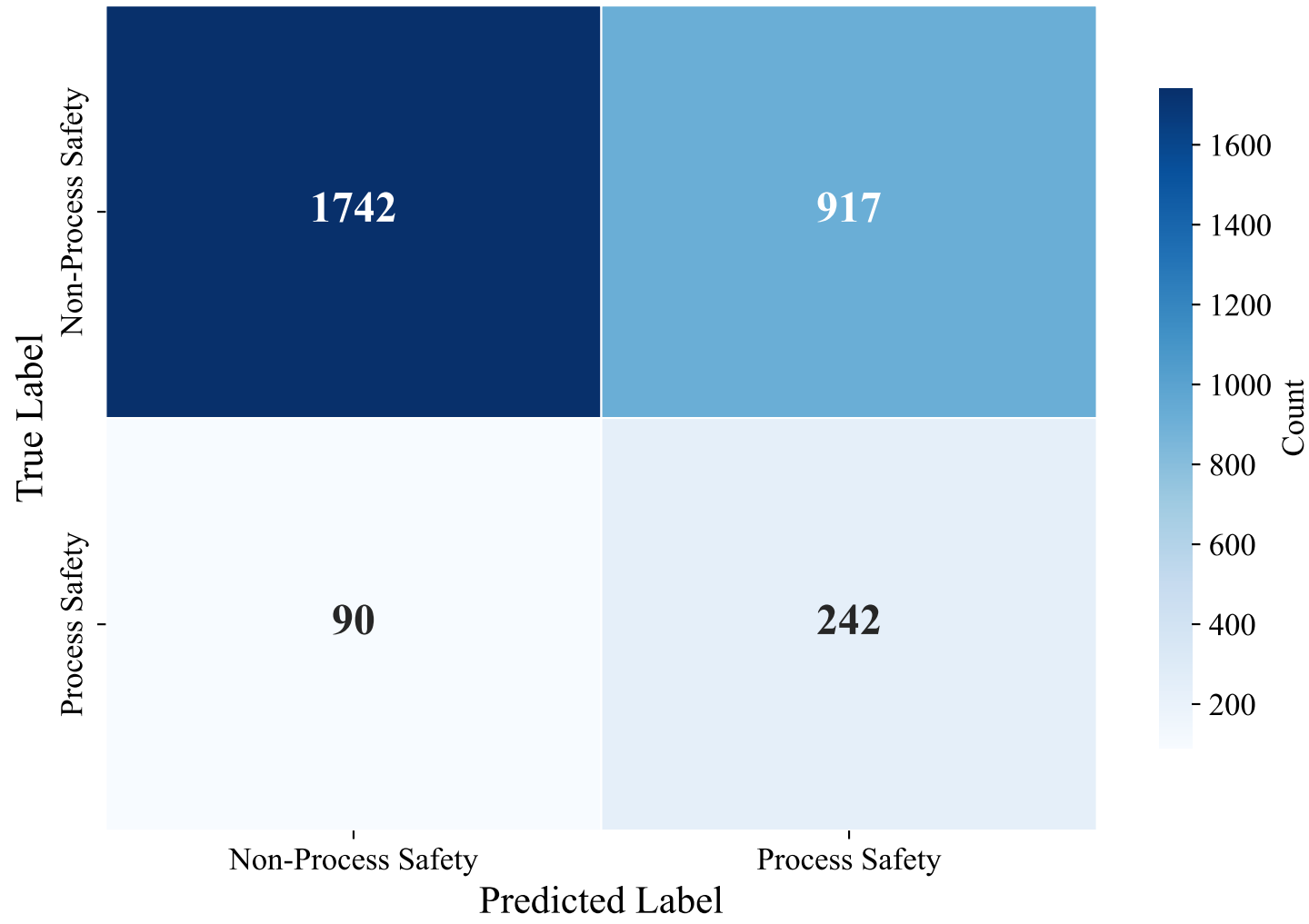
Confusion Matrix — GERMAN_MANUAL (bert-base-multilingual-uncased, Random_Forest)
