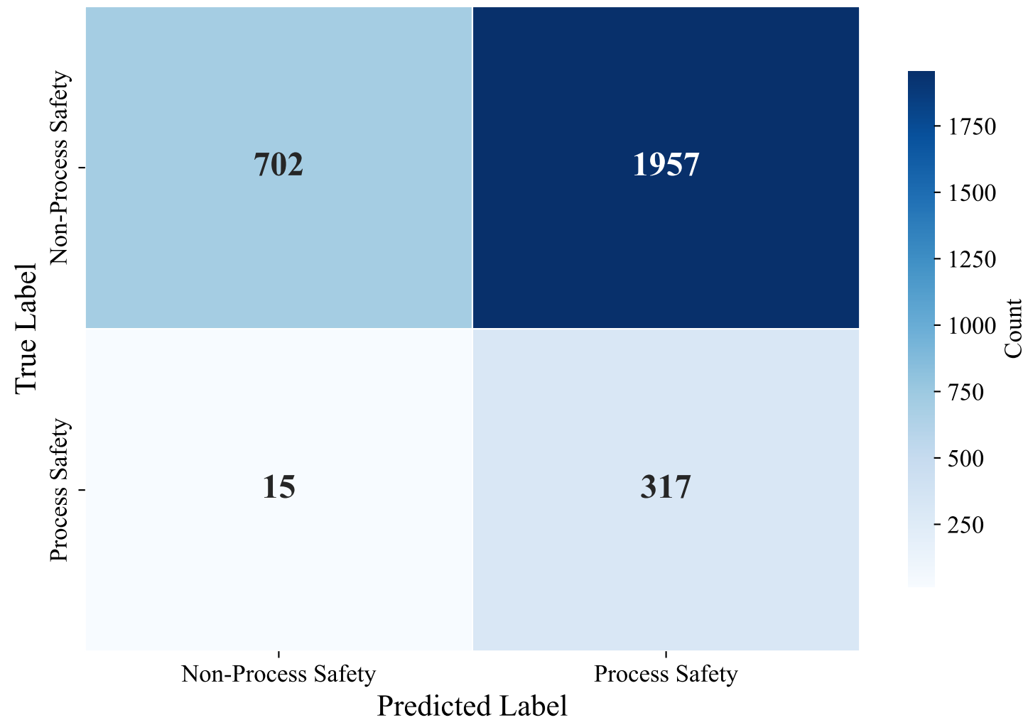
Confusion Matrix — GERMAN_MANUAL (paraphrase-multilingual-mpnet-base-v2, Random_Forest_Optimized)
