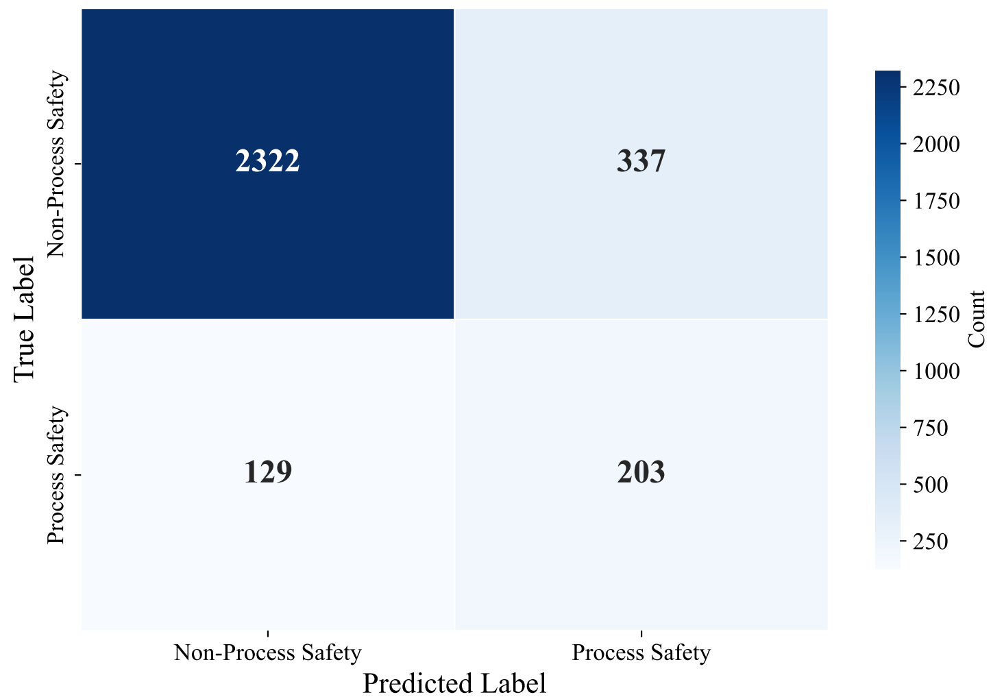
Confusion Matrix — GERMAN_MANUAL (paraphrase-multilingual-mpnet-base-v2, XGBoost)
