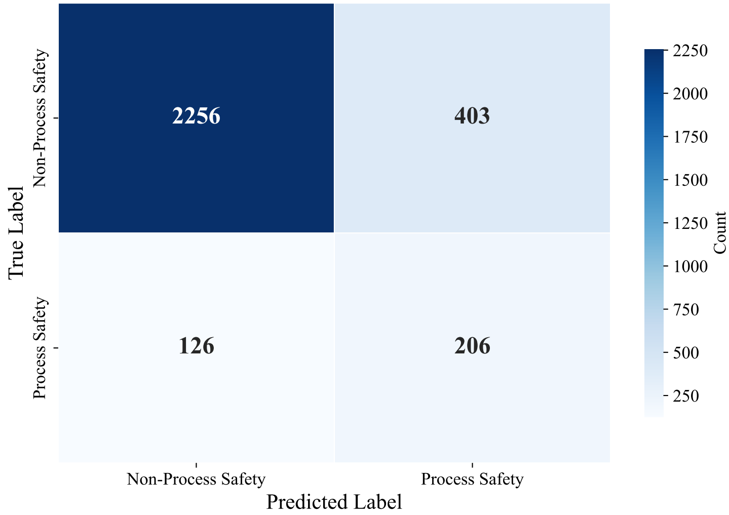
Confusion Matrix — GERMAN_MANUAL (xlm-roberta-base, Voting_Ensemble)
