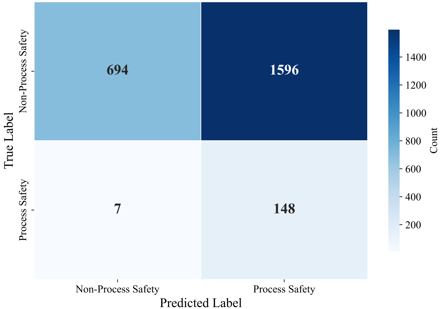
Confusion Matrix — SWEDISH_MANUAL (xlm-roberta-base, Random_Forest_Optimized)
