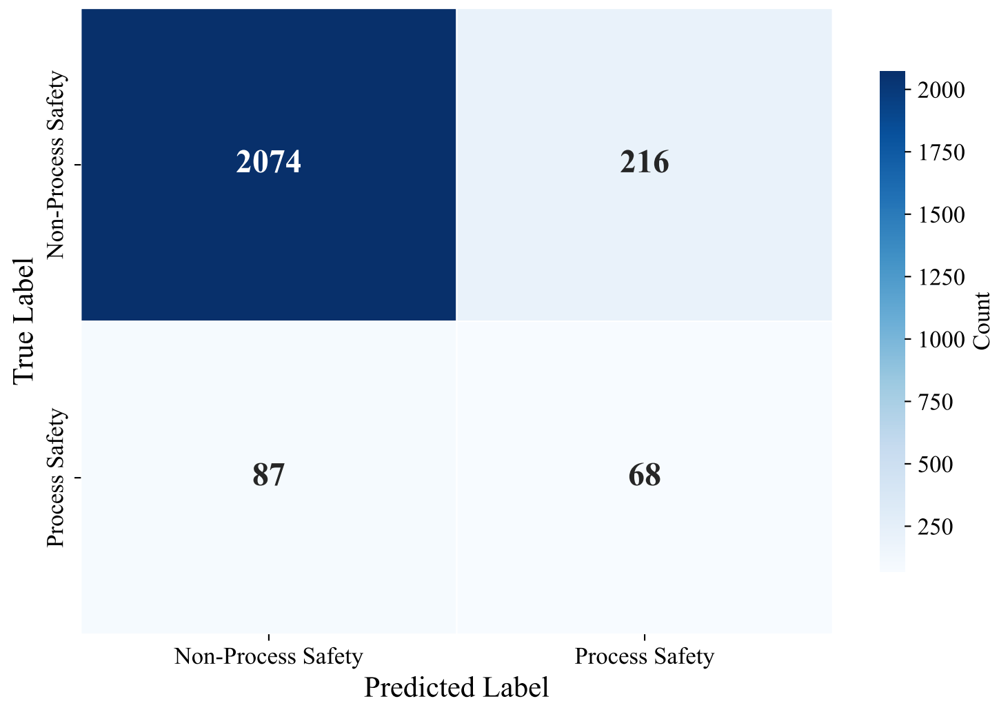
Confusion Matrix — SWEDISH_MANUAL (xlm-roberta-base, XGBoost_Optimized)
