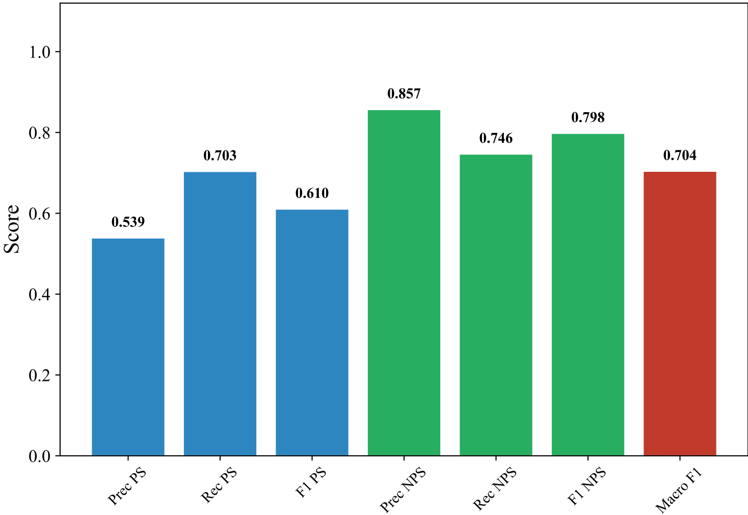
Classification Metrics — DUTCH_MANUAL (xlm-roberta-base, LightGBM)
