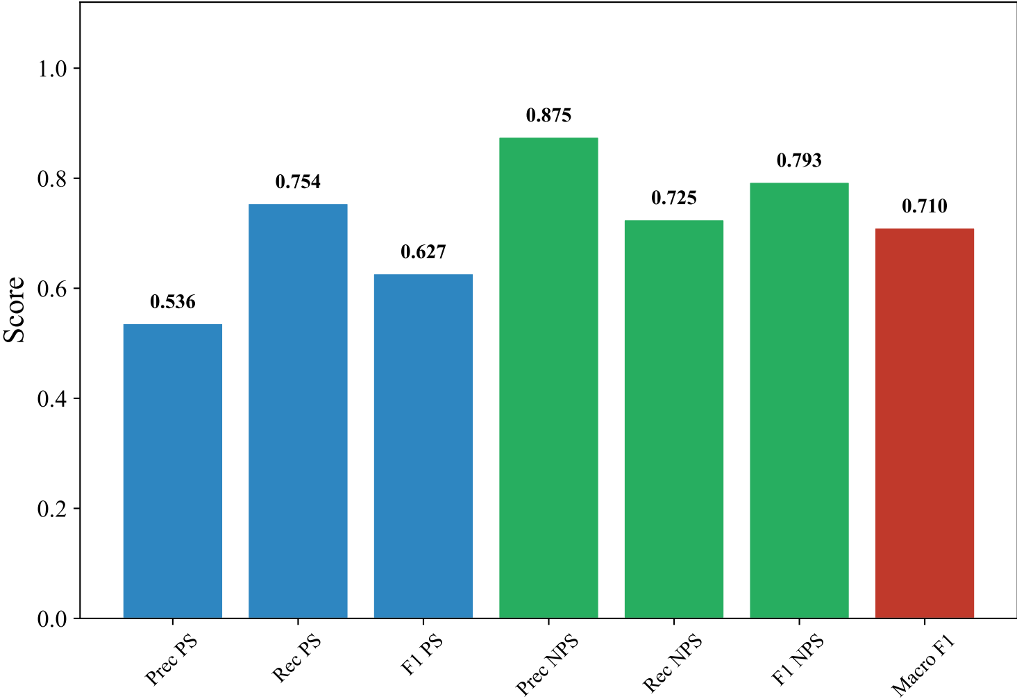
Classification Metrics — DUTCH_MANUAL (xlm-roberta-base, Voting_Ensemble)
