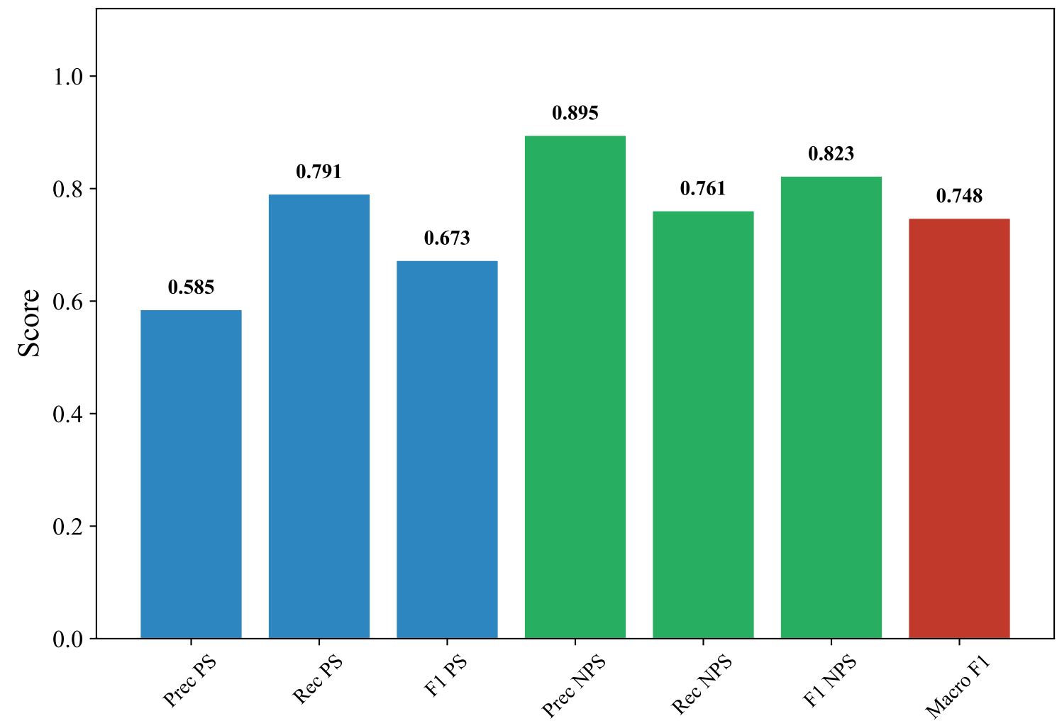
Classification Metrics — ENGLISH_MANUAL (bert-base-multilingual-uncased, LightGBM_Optimized)
