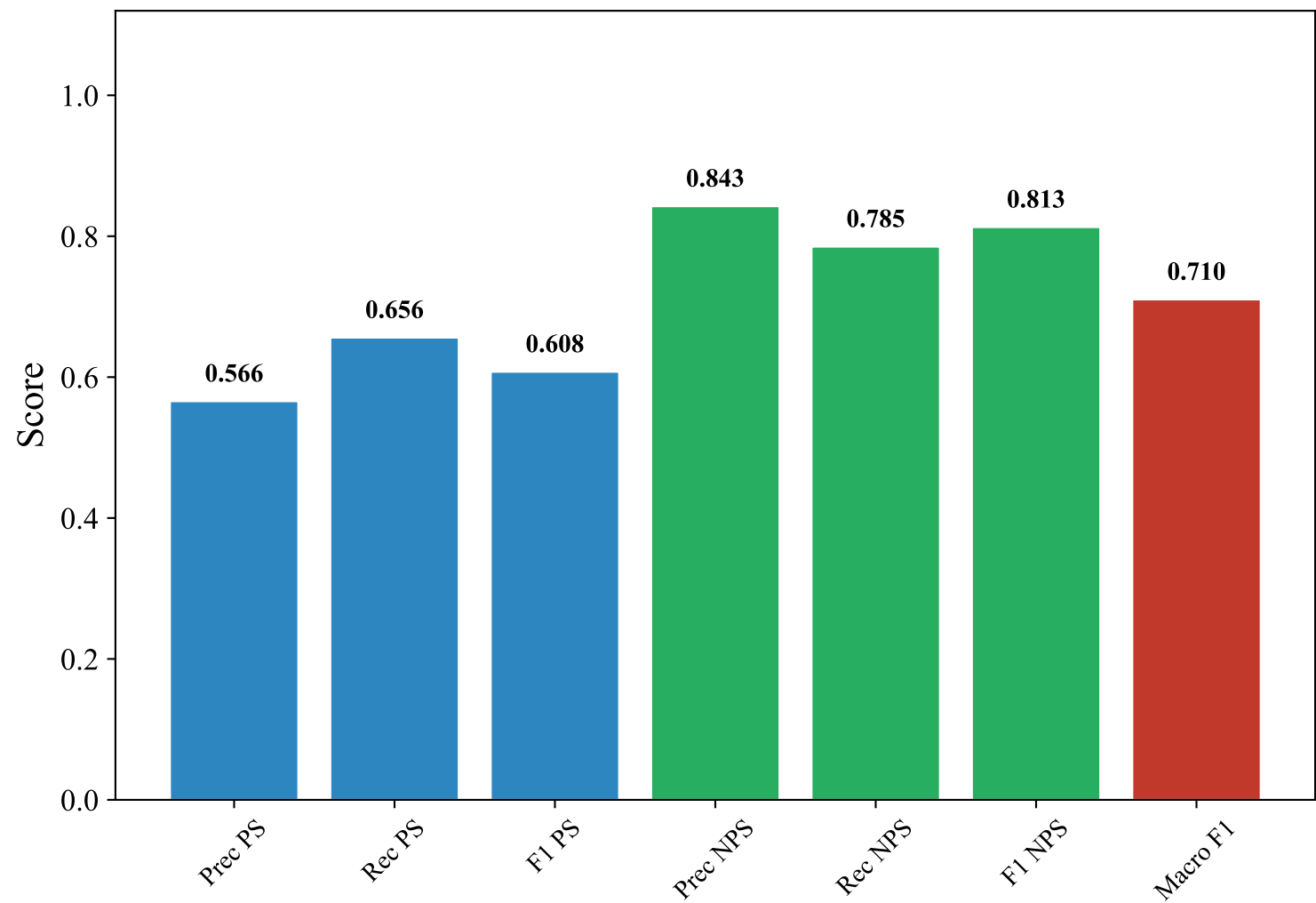
Classification Metrics — ENGLISH_MANUAL (bert-base-multilingual-uncased, SVM)
