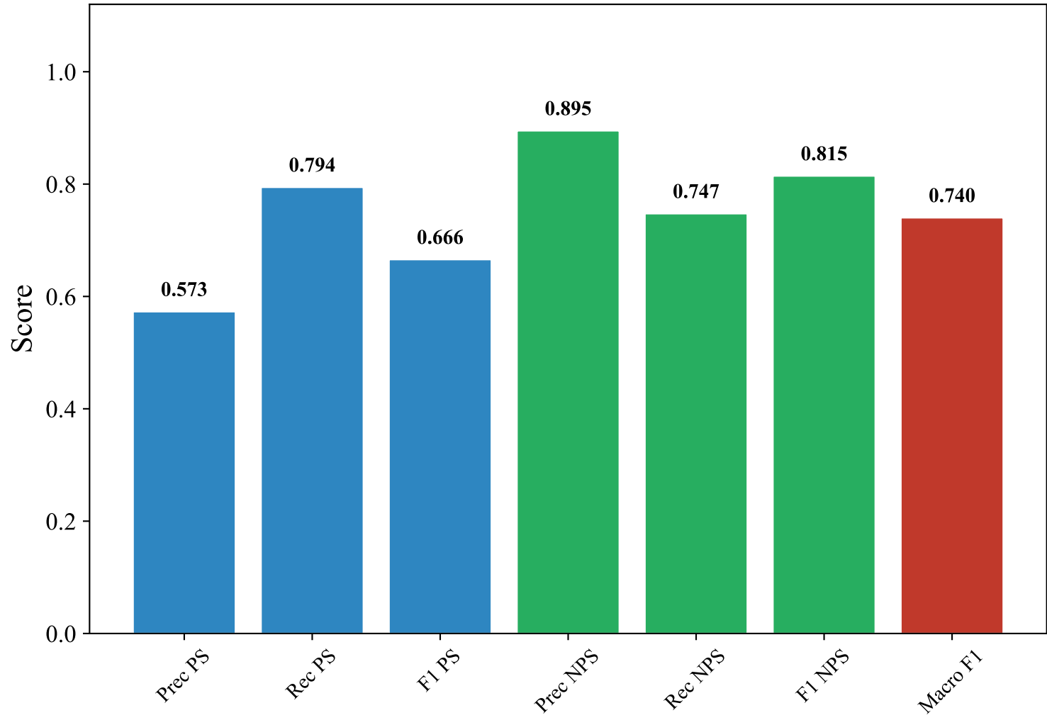
Classification Metrics — ENGLISH_MANUAL (bert-base-multilingual-uncased, Voting_Ensemble)
