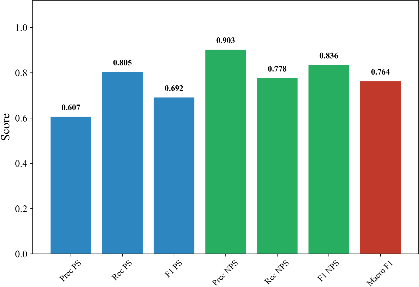
Classification Metrics — ENGLISH_MANUAL (paraphrase-multilingual-mpnet-base-v2, LightGBM_Optimized)
