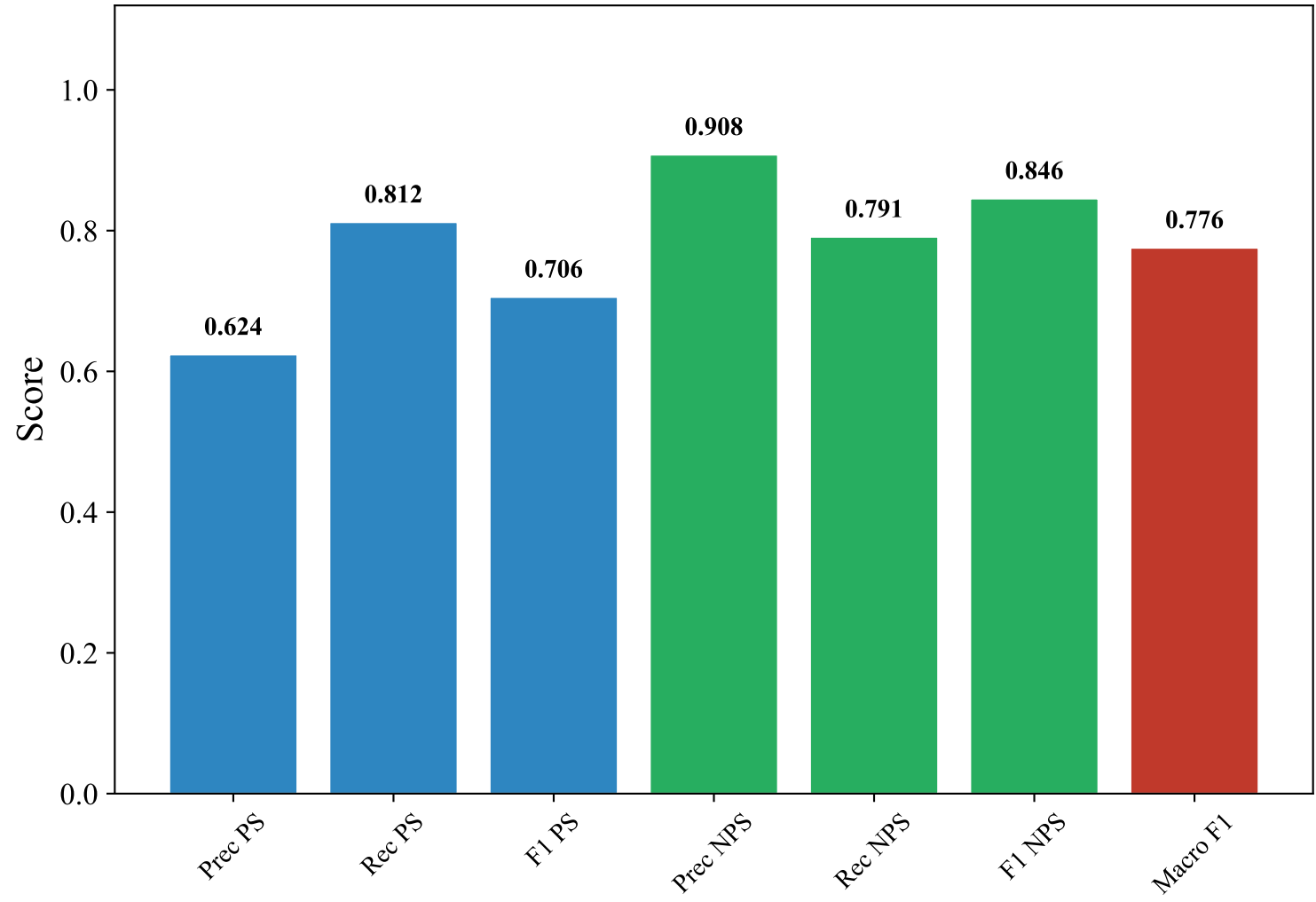
Classification Metrics — ENGLISH_MANUAL (paraphrase-multilingual-mpnet-base-v2, XGBoost)
