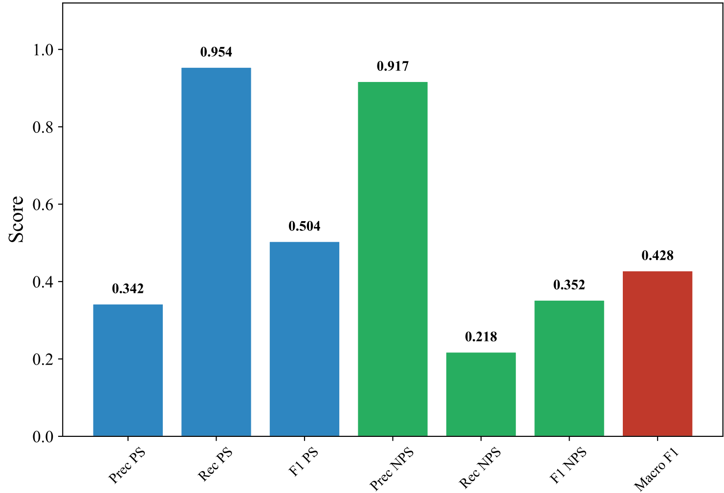
Classification Metrics — ENGLISH_MANUAL (xlm-roberta-base, Random_Forest_Optimized)
