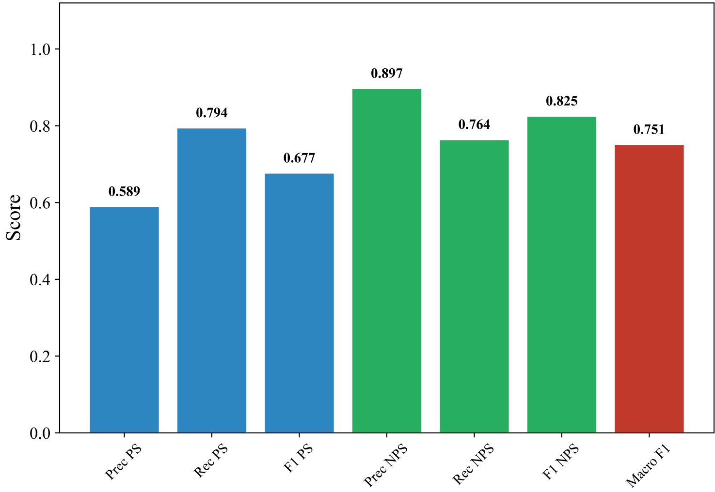
Classification Metrics — ENGLISH_MANUAL (xlm-roberta-base, Voting_Ensemble)
