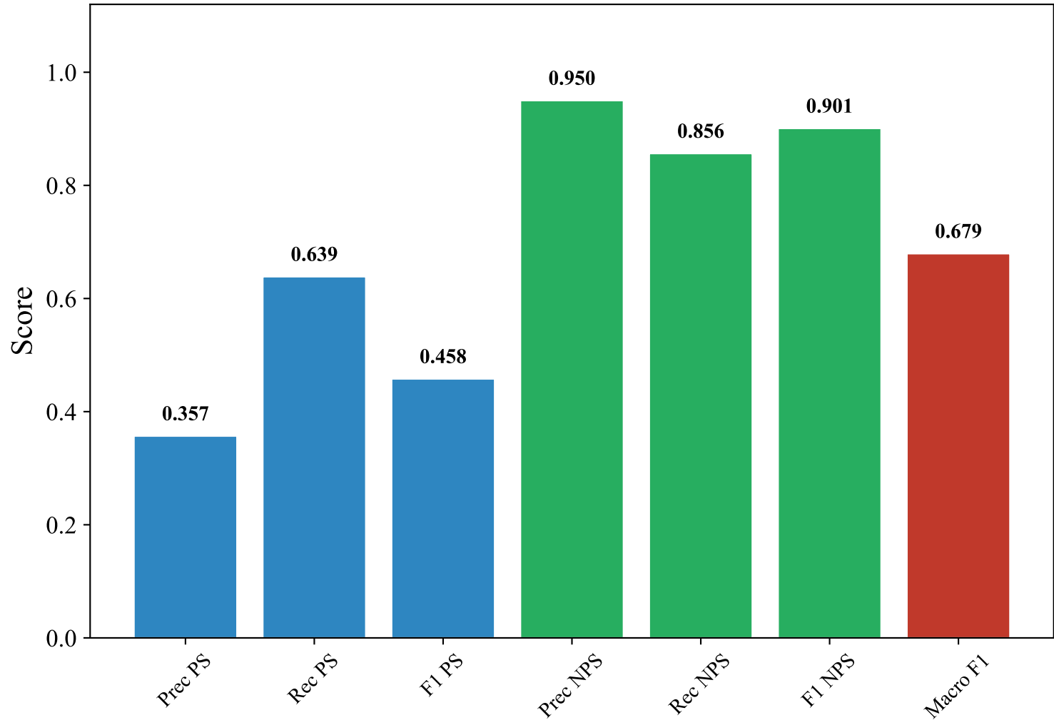
Classification Metrics — GERMAN_MANUAL (bert-base-multilingual-uncased, Voting_Ensemble)
