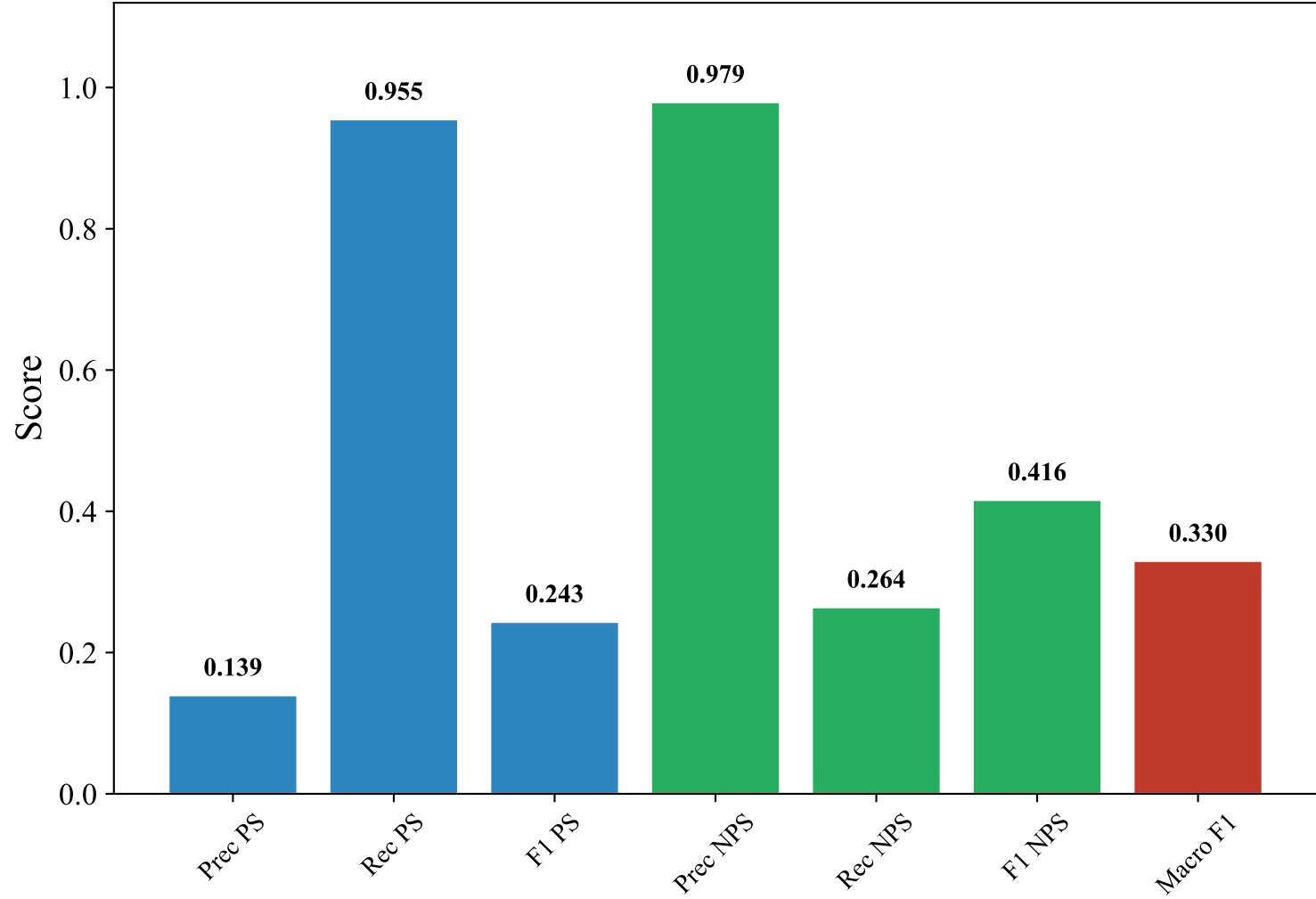
Classification Metrics — GERMAN_MANUAL (paraphrase-multilingual-mpnet-base-v2, Random_Forest_Optimized)
