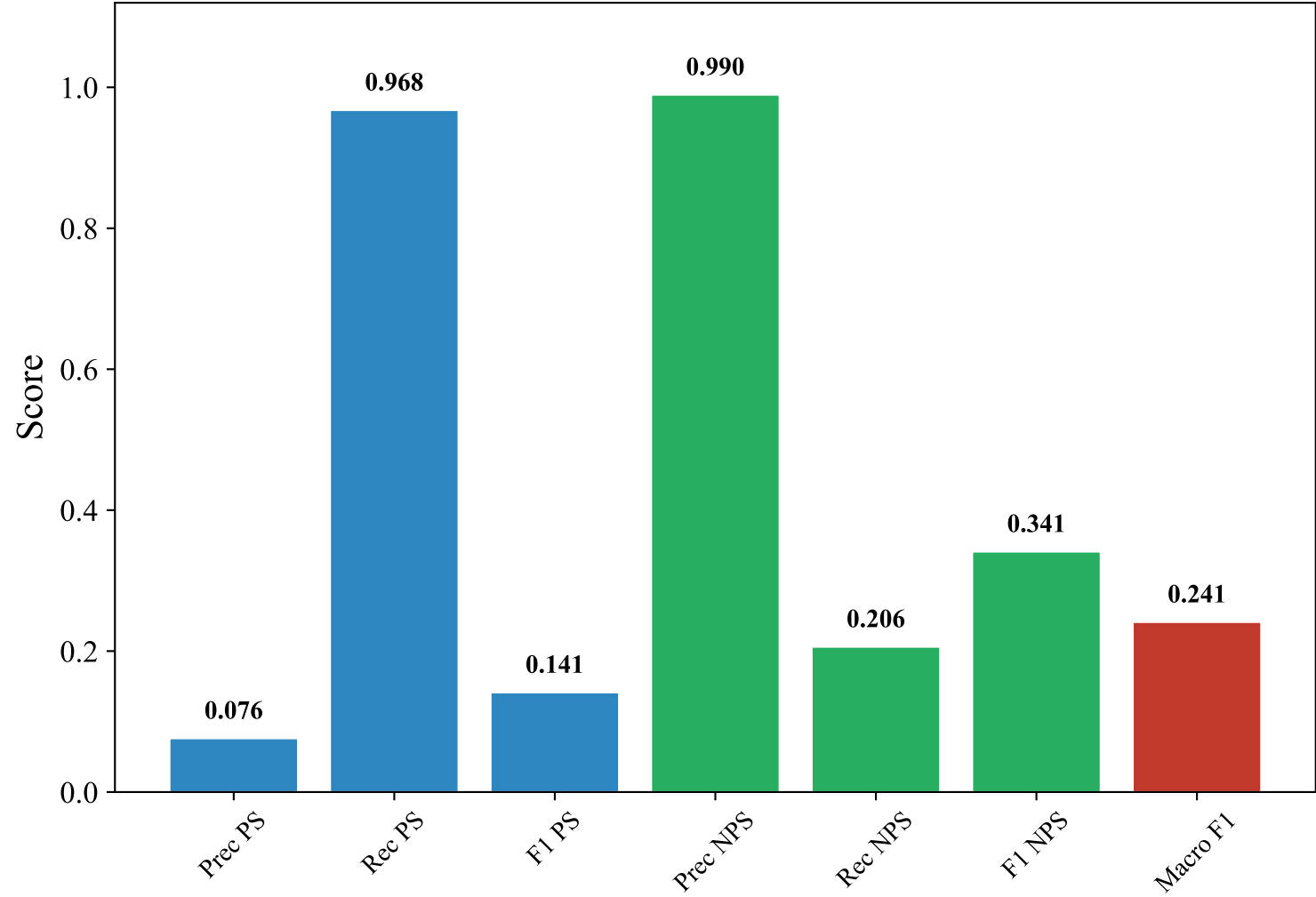
Classification Metrics — SWEDISH_MANUAL (bert-base-multilingual-uncased, Random_Forest_Optimized)
