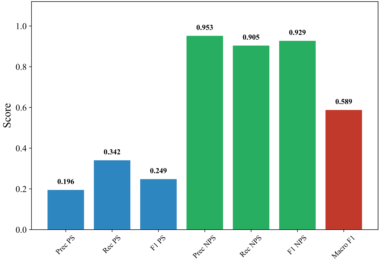
Classification Metrics — SWEDISH_MANUAL (bert-base-multilingual-uncased, XGBoost_Optimized)
