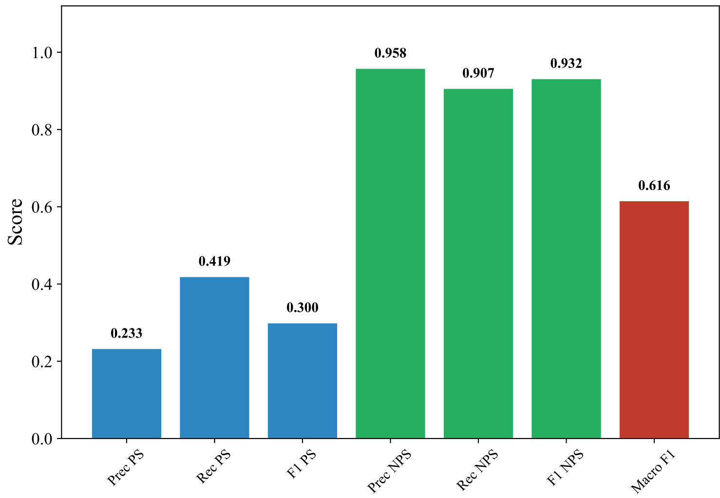
Classification Metrics — SWEDISH_MANUAL (xlm-roberta-base, LightGBM_Optimized)
