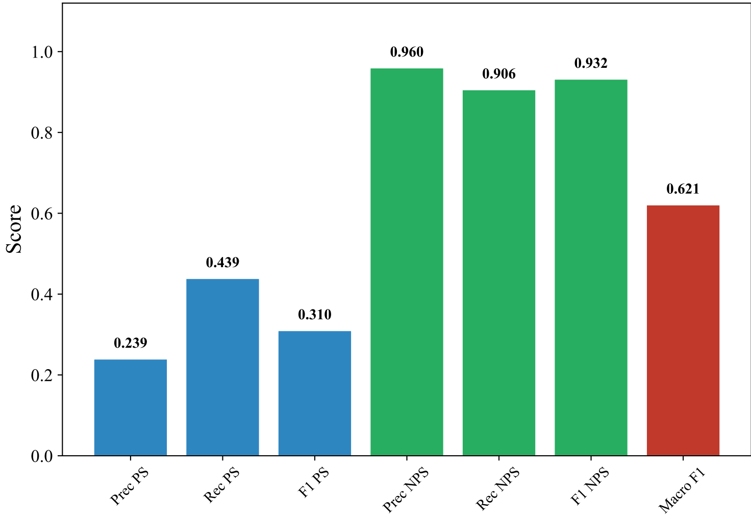
Classification Metrics — SWEDISH_MANUAL (xlm-roberta-base, XGBoost)
