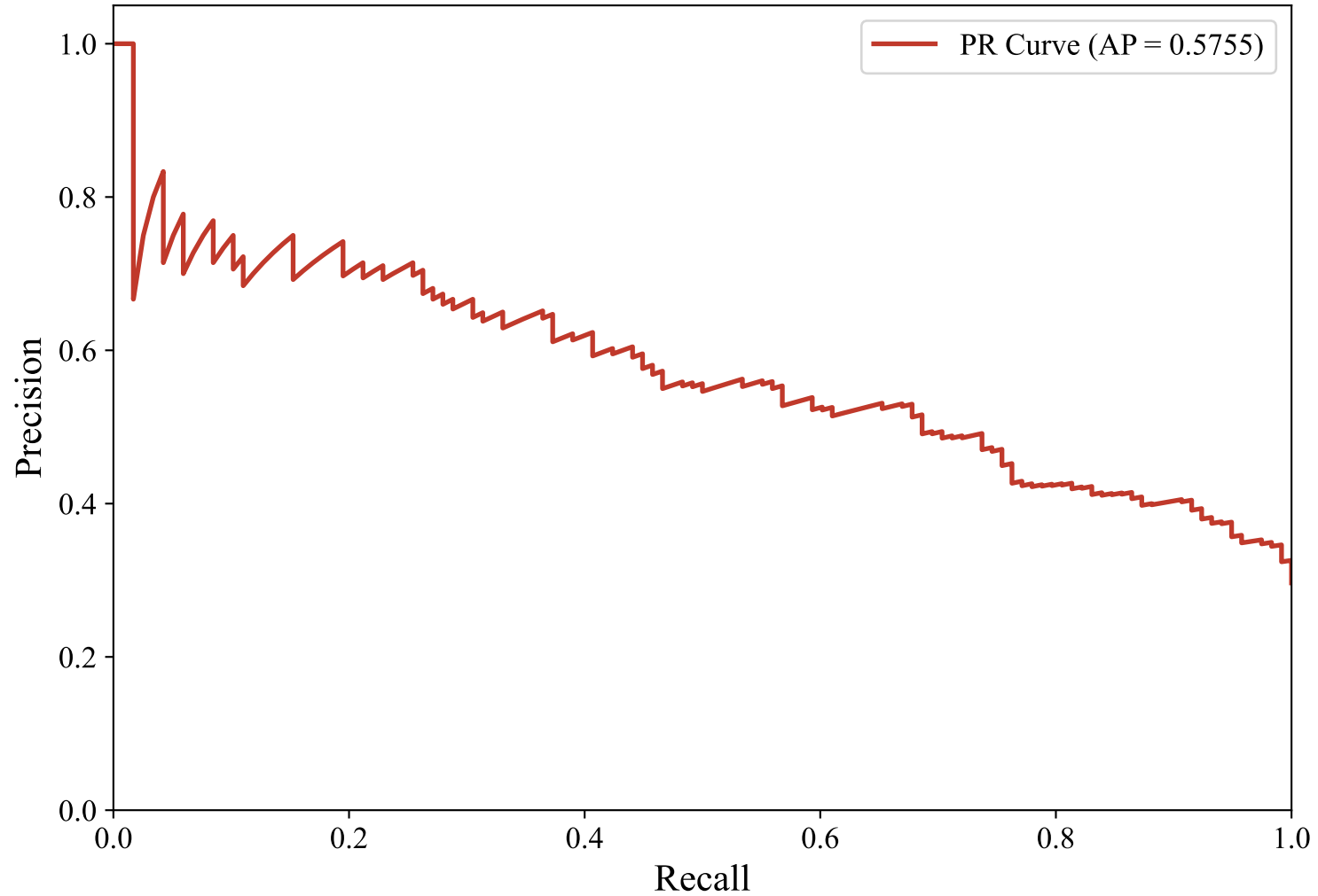
Precision-Recall Curve — DUTCH_MANUAL (bert-base-multilingual-uncased, LightGBM)
