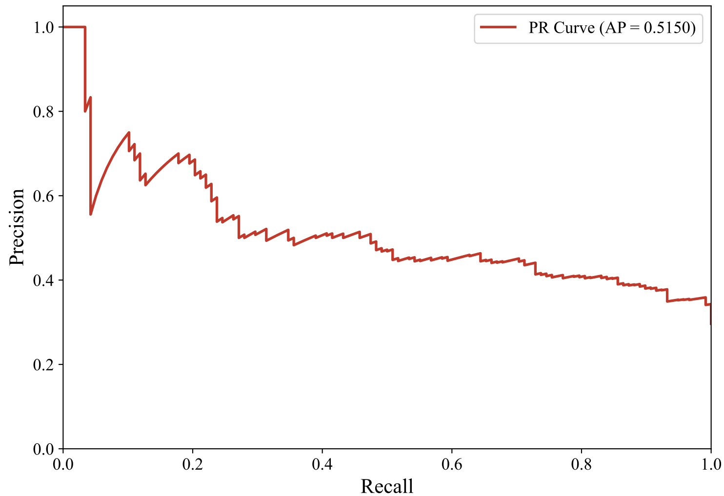
Precision-Recall Curve — DUTCH_MANUAL (bert-base-multilingual-uncased, Random_Forest)
